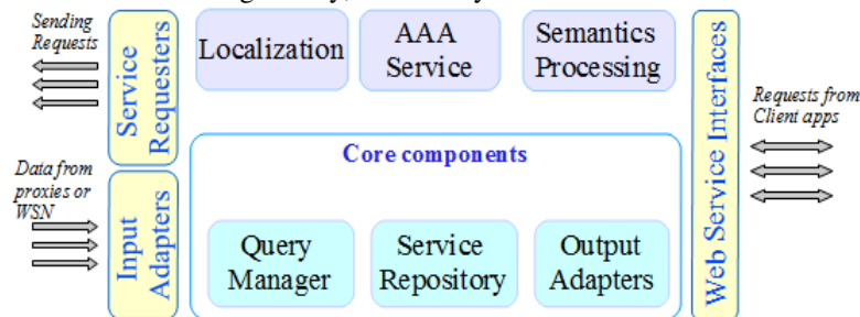
Fig. 3. The Architecture of Middleware
